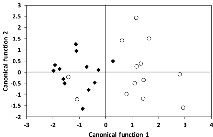
Fig. 2. Graphic representation of separation of fields into zebra chip occurrence class of 1 (open circles) or 2 (closed diamonds) based on selected variables using canonical discriminant function analysis.
